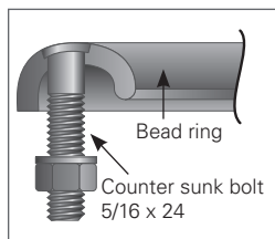
BEAD RING-TYPE PART
